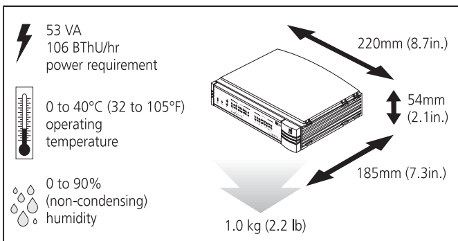
OfficeConnect Dual Speed Hub 16
