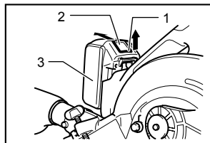
1. Red part 2. Button 3. Battery cartridge
