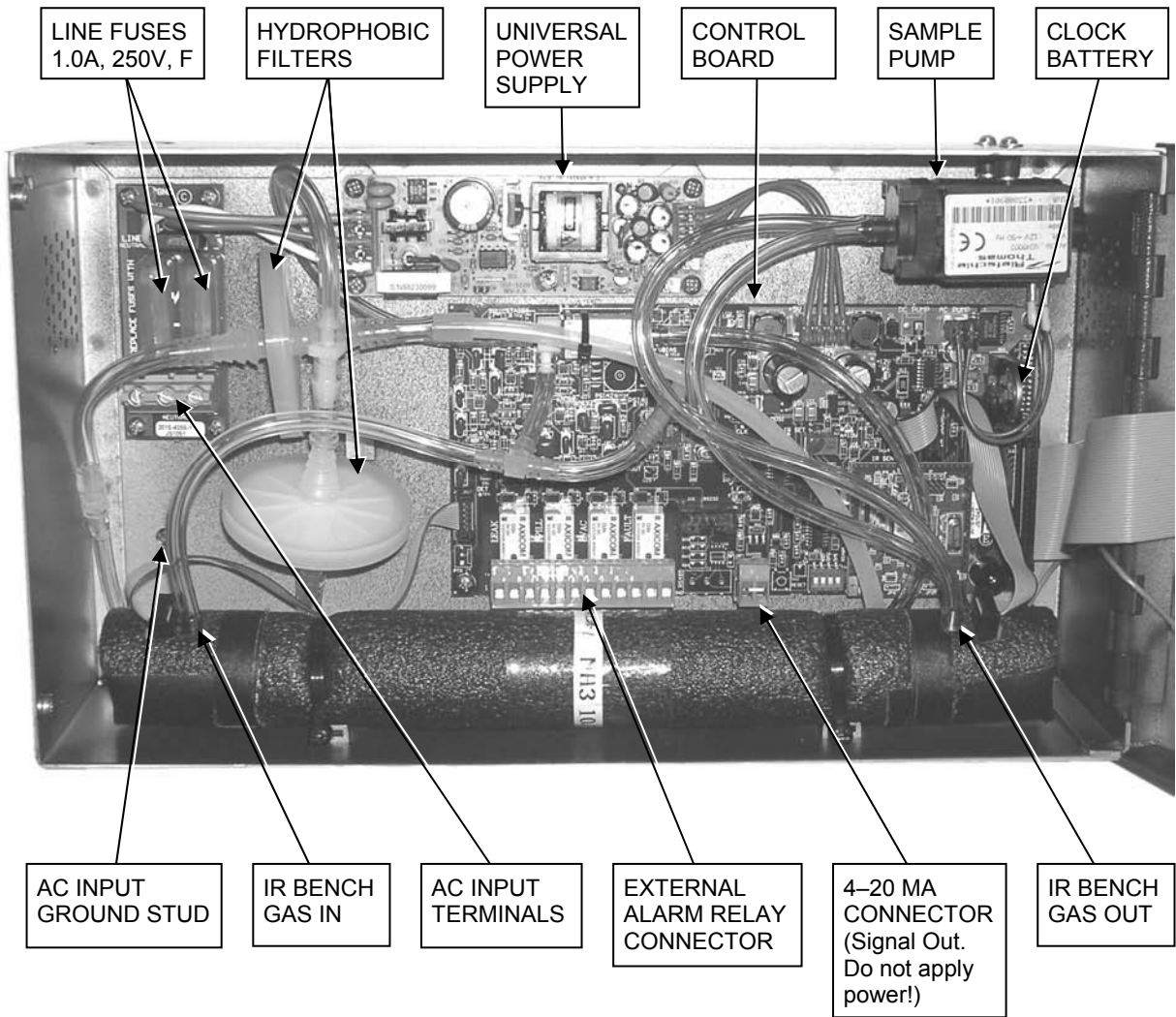
Interior Schematic
