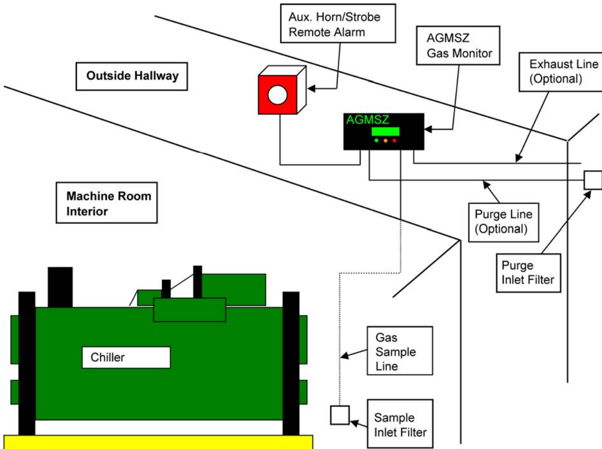
AGMSZ Refrigerant Gas Leak Monitor Mechanical Room Placement
