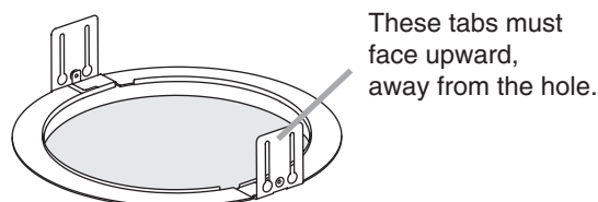
HY-RR2 placed on ceiling panel
