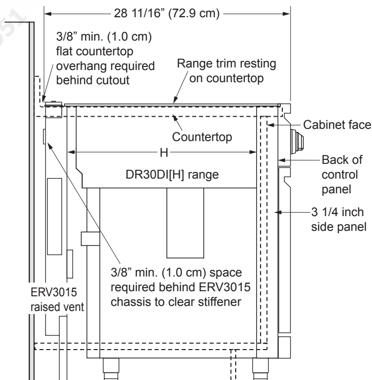
Side View
