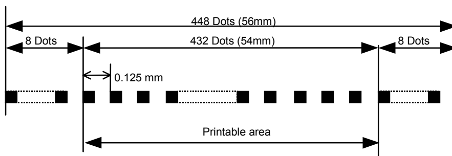
Figure 3-1 Heat Element Dimensions (LTPF247)
