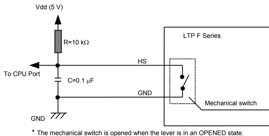
Figure 3-16 Sample External Circuit of the Platen Position Detector
