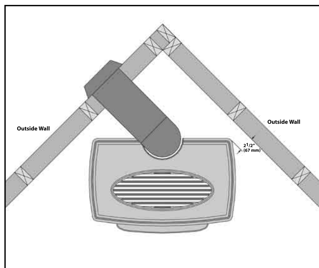
Figure 22: Corner installation top vented.
