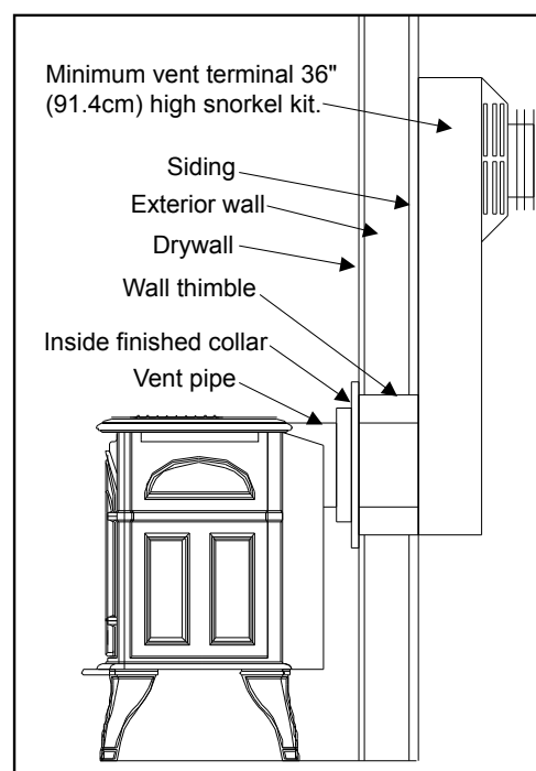
Figure 36: Installation for Rear Vented; 30,000 Btu/hr.
