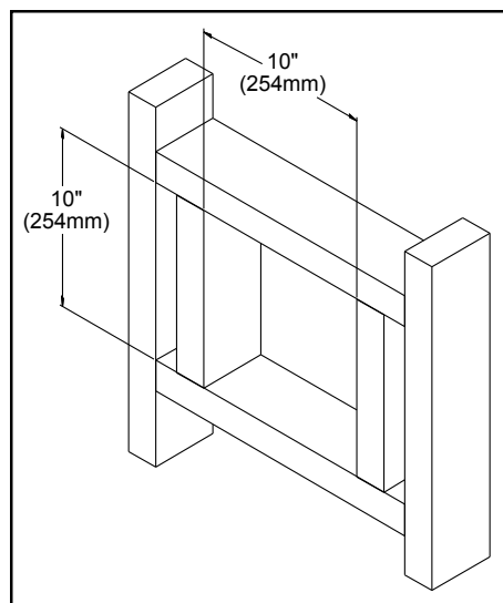
Figure 17: Wall Framing Hole for Horizontal Installation.
