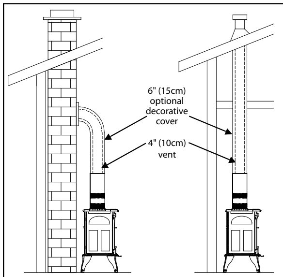
Figure 40: Unit top venting styles.
