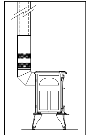
Figure 41: Unit rear venting style.
