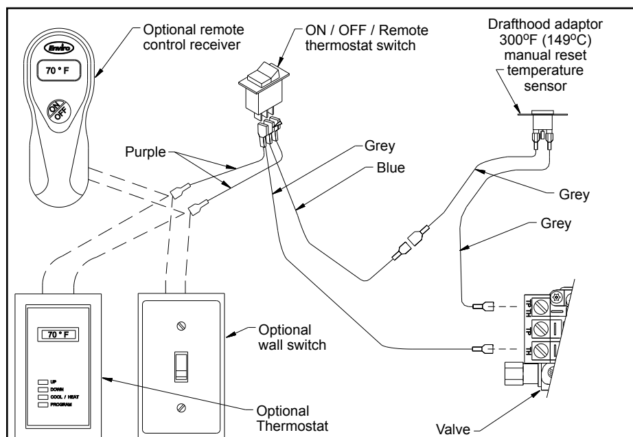
Figure 39: Wiring Diagram for Electrical Connection.
