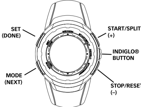
Button functions shown with secondary functions in parentheses
