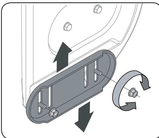
Figure 5-5 - Reversible Steel Skid Shoe
