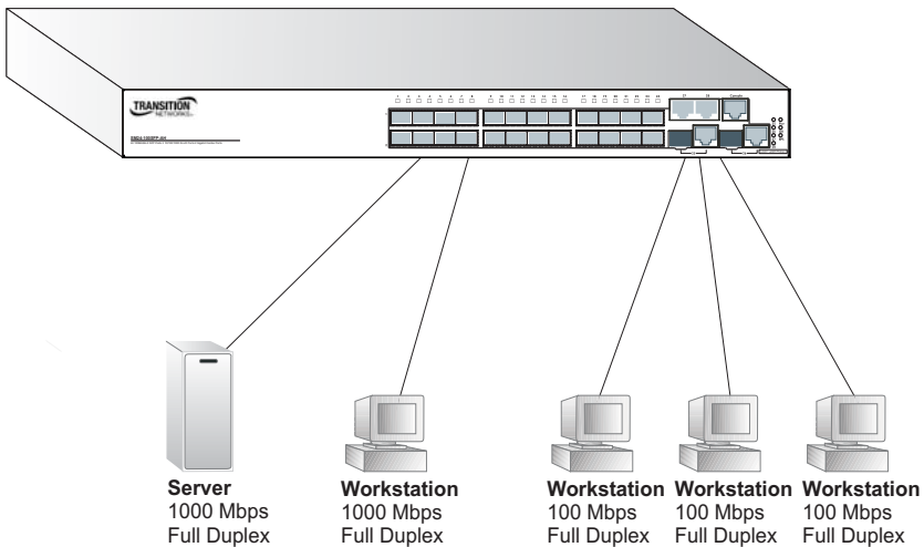
Figure 2-1. Collapsed Backbone
