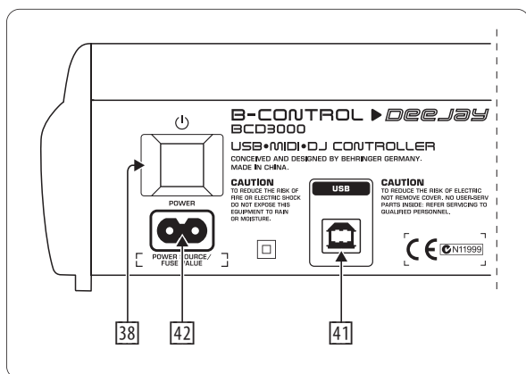
Fig. 3.3: POWER switch, mains and USB connectors
