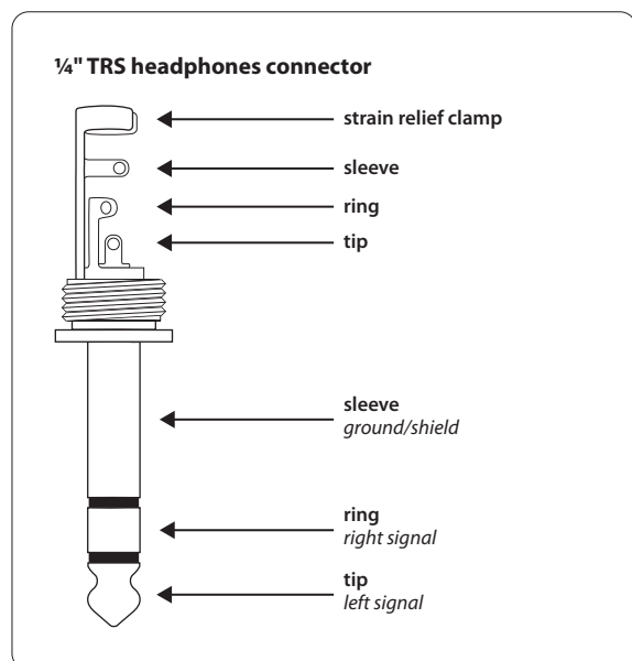
Fig. 7.2: 1/4" TRS headphones connector
