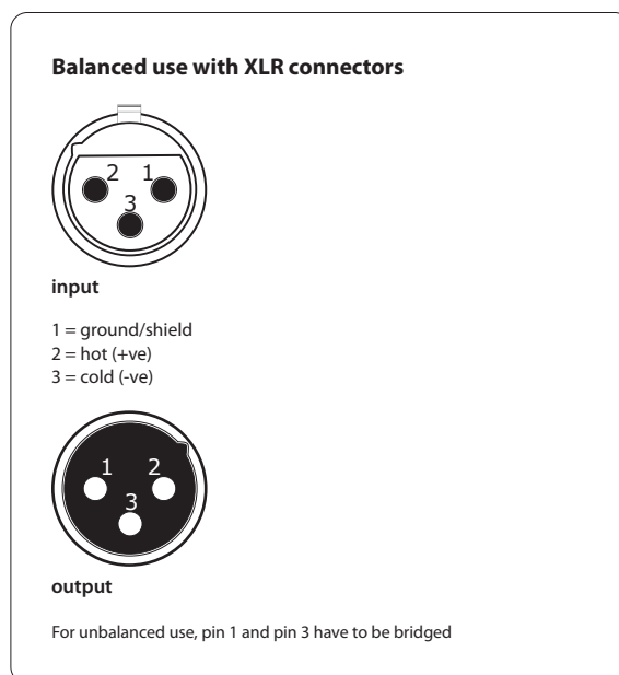
Fig. 7.1: XLR connector
