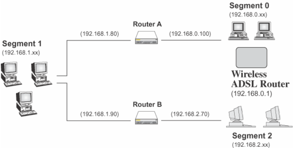
Figure 71: Routing Example
