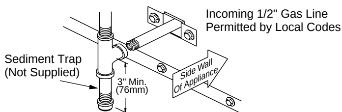
Figure 18 - Sediment Trap
