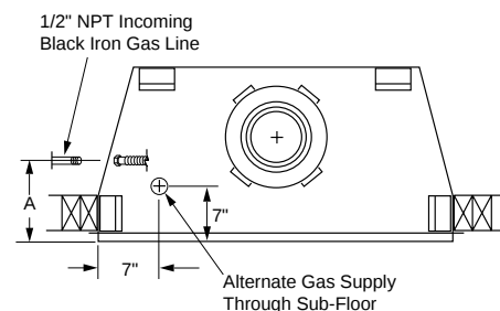
Figure 16 - Manual Shutoff Valve Installation
