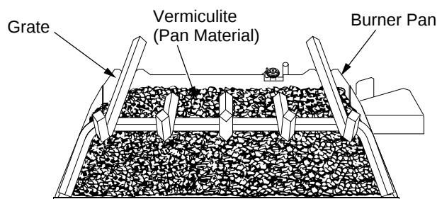
Figure 20 - Fill Entire Burner Pan with Vermiculite
