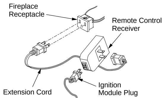
Figure 14 - Installing the WRC Remote Receiver
