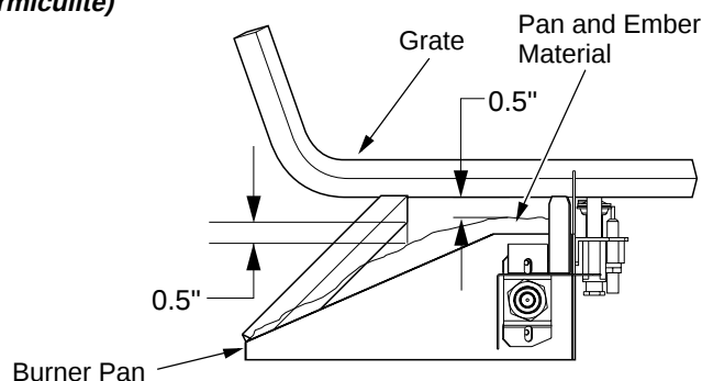
Figure 21 - Ember Material on Surface of Pan Material (Vermiculite)
