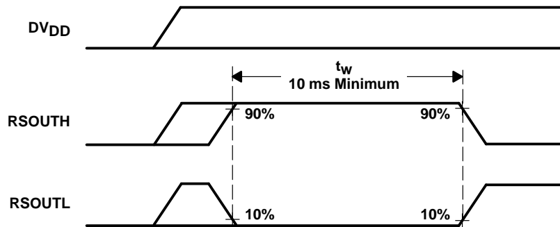
Figure 4–12. Power-On Reset Timing
