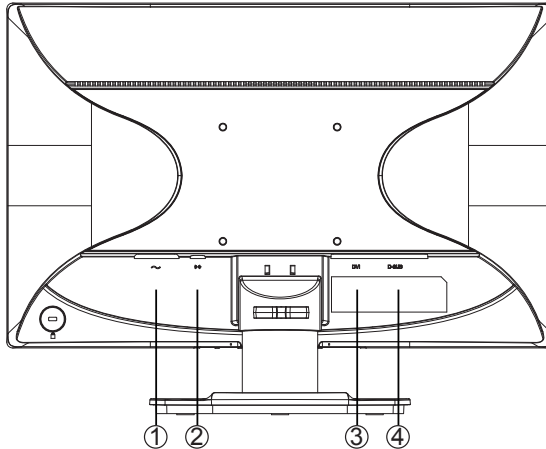
Figure 2 Connecting Cables
