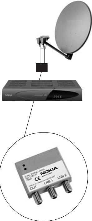
DiSEqC switch with 2 inputs
