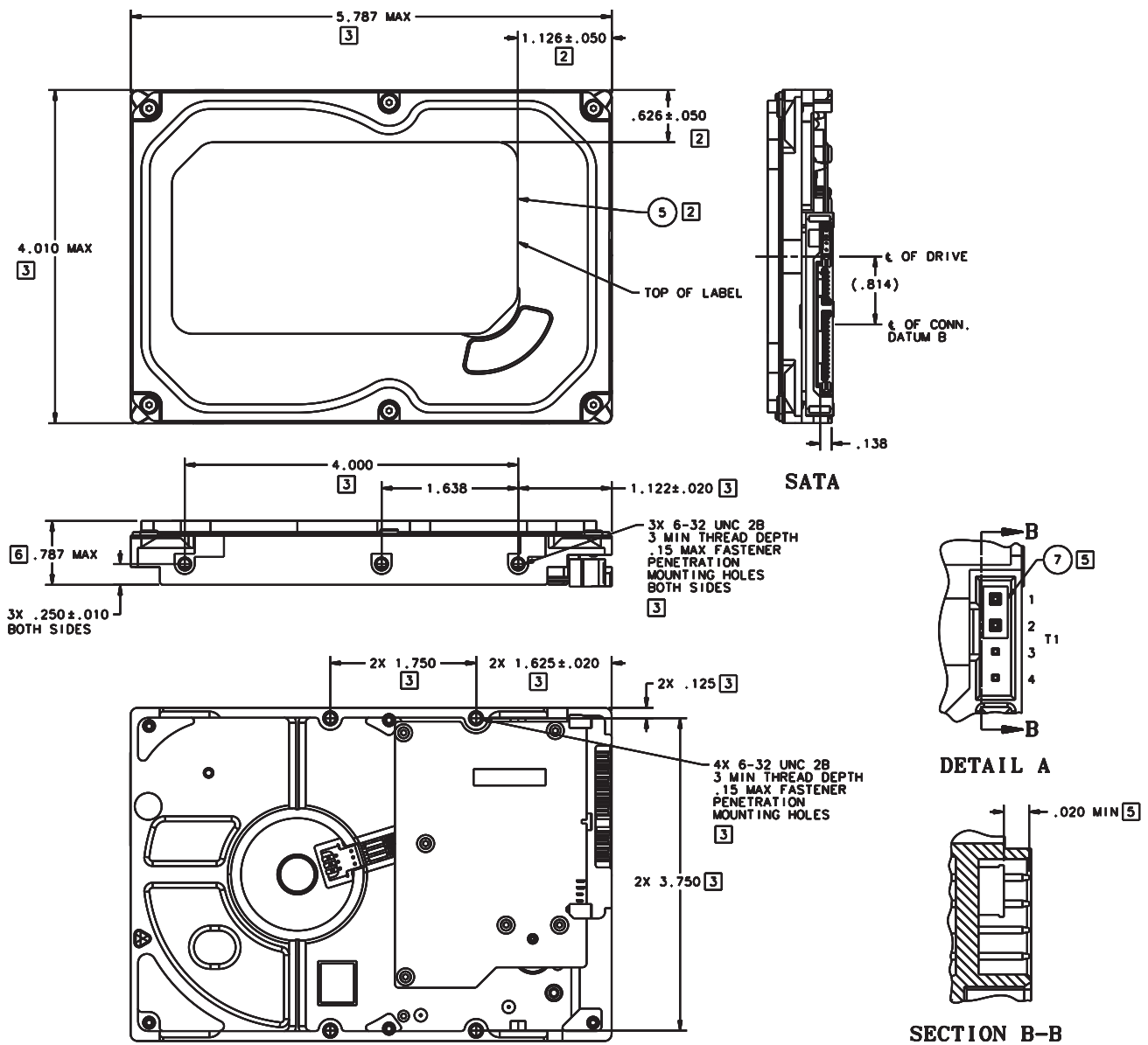
Figure 4. Mounting dimensions (320 & 160 GB models)
