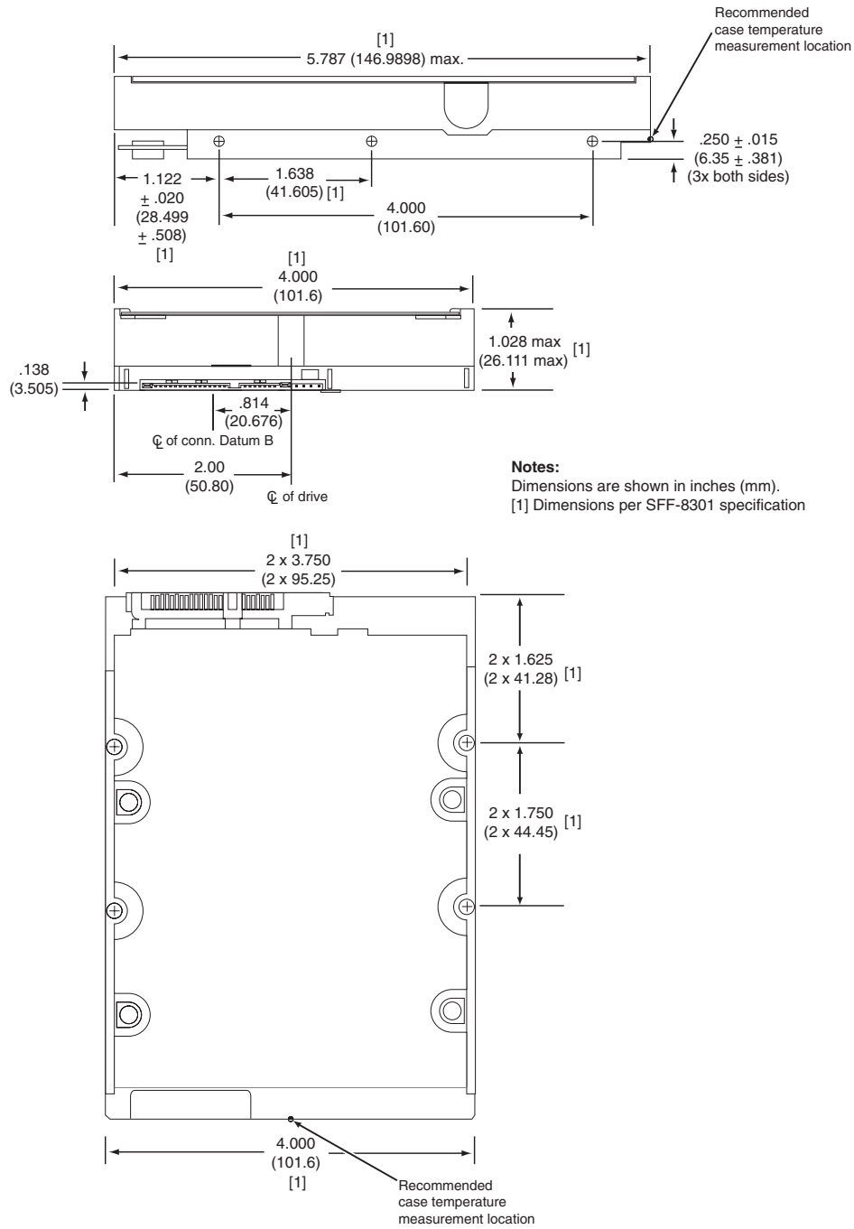
Figure 3. Mounting dimensions (1000 & 640 GB models)
