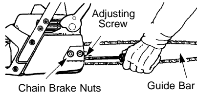
Adjusting Screw - 1/4 Turn
