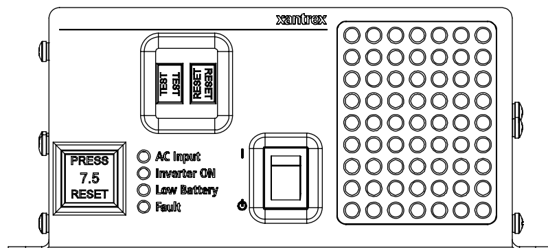
Figure 3-1 Front Panel
