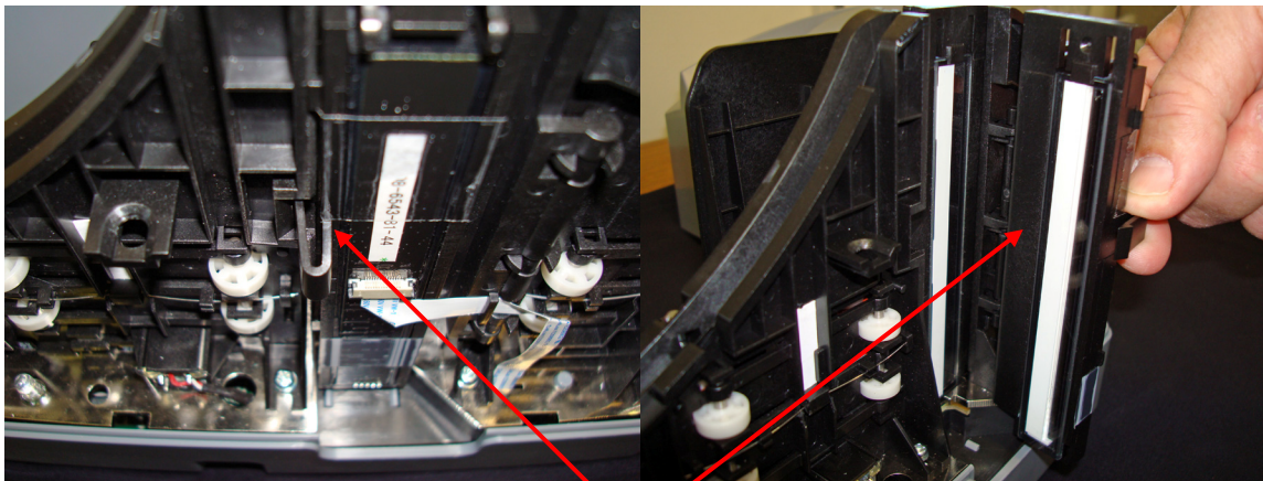
Fig.10 Outer camera door. Pinch latch to pivot door open.
