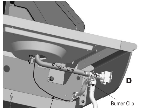
Correctly assembled burner-to-valve engagement
