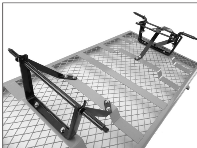
Figure 2. Rear and front axle assemblies
