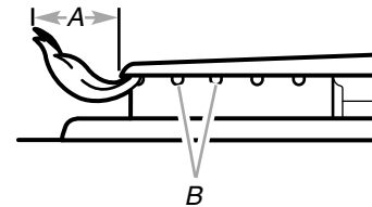
A. 1 to 1 1/2" (25 to 38 mm) B. Burner ports
