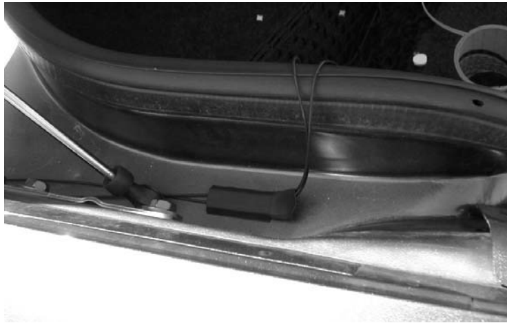
Figure 15: Cable routing along the trunk rubber molding
