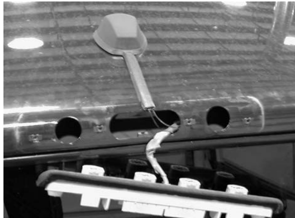
Figure 30: Brakelight cavity
