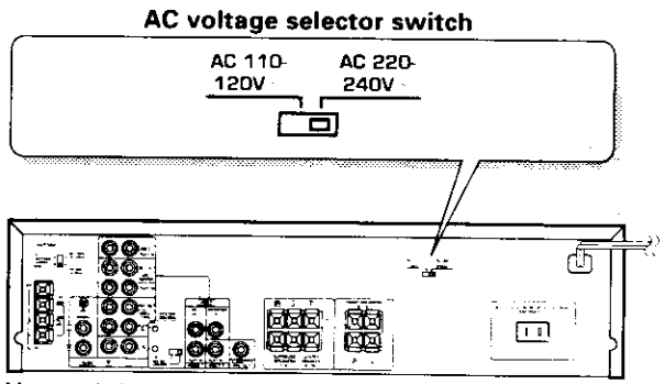
Move switch lever to match your line voltage with a small screwdriver or other pointed tool.
