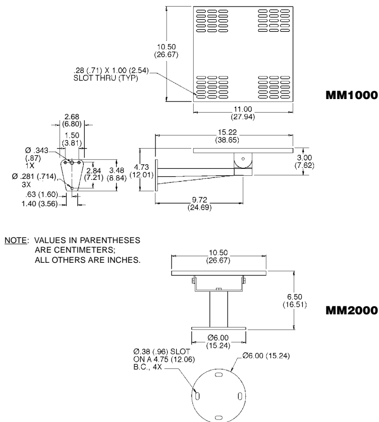
Figure 3. MM1000/MM2000 Dimensions
