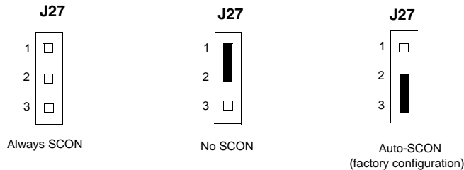
Figure 1-11 J27 Settings
