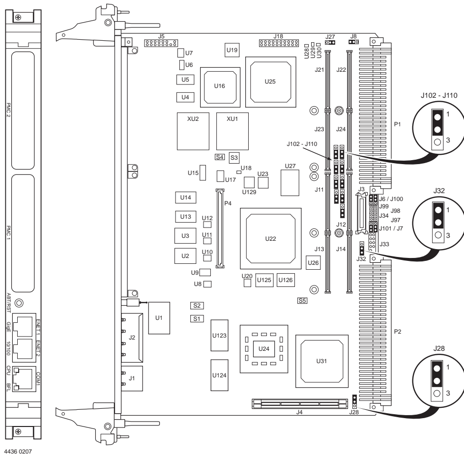
Figure B-2 Thermally Significant Components—Primary Side
