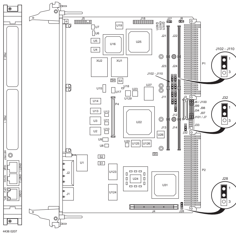
Figure 1-1 MVME5500 Board Layout
