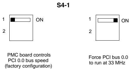
Figure 1-10 S4-1 Settings
