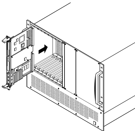
Figure 1-17 Installation into a Typical VME Chassis
