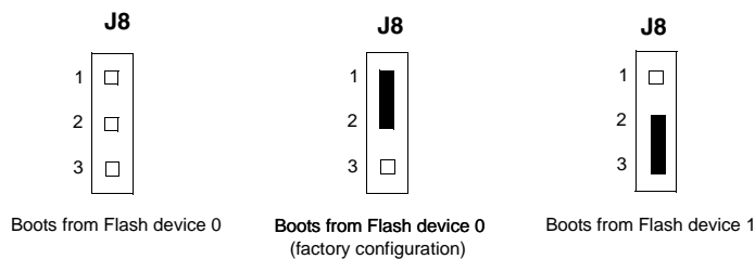
Figure 1-5 J8 Settings
