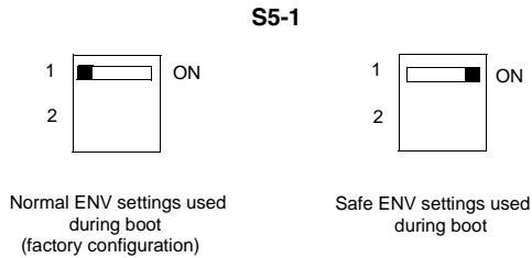
Figure 1-7 S5-1 Settings
