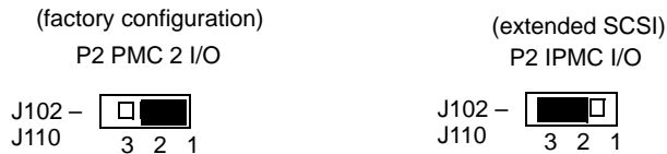
Figure 1-4 J102 - J110 Settings
