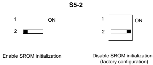
Figure 1-9 S5-2 Settings
