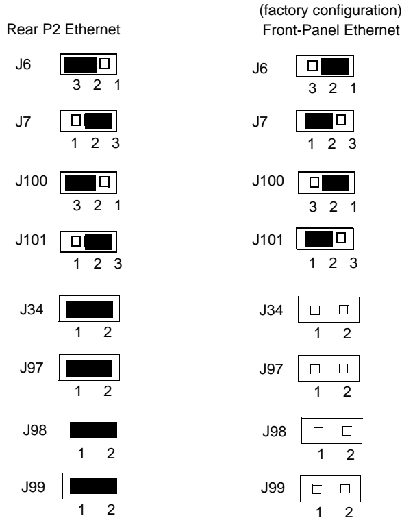
Figure 1-2 Front Panel and Rear P2 Ethernet Settings
