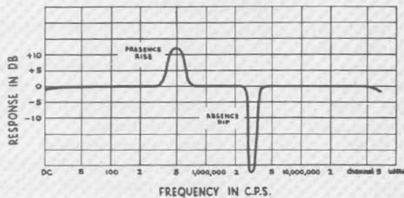
FIGURE 3 — Frequency Response at 791-watt Level
