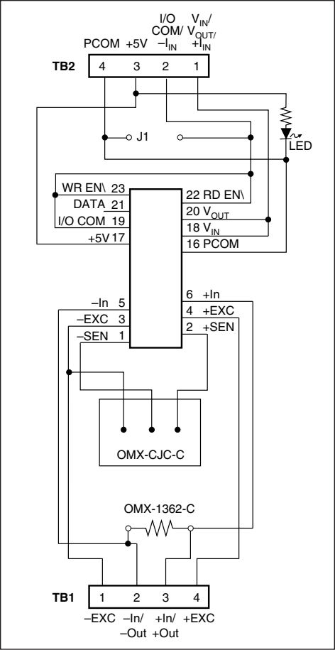
FIGURE 11. OM5-BP-SKT-C Schematic.
