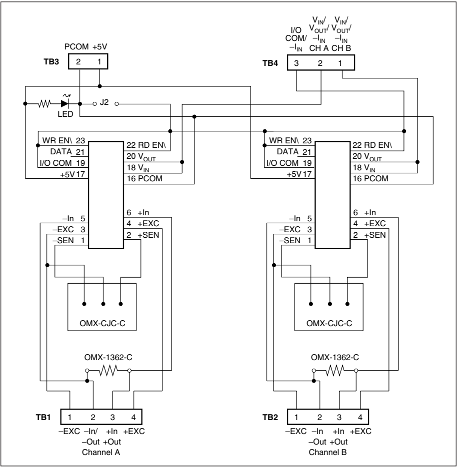
FIGURE 12. OM5-BP-2-C Schematic.
