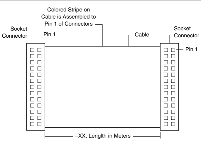
FIGURE 21. OMX-1315-XX-C System Interface Cable.
