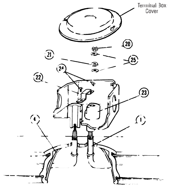
Figure 10 — Center Element
