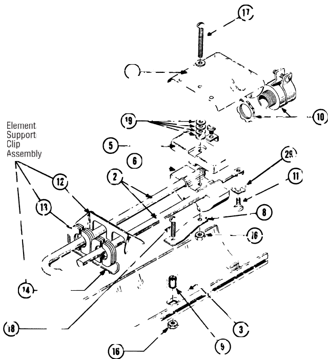
Figure 9 — End Element
