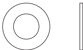
[18#] \varnothing 13 * \varnothing 24 * 1.5 22pcs
