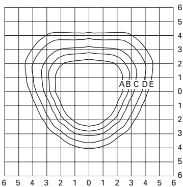
ACN17M3C.IES 175-Watt MH 14,000-Lumen Clear ED-28 Lamp Type III Cutoff
