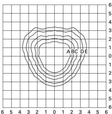
ACN15S3C.IES 150-Watt HPS 16,000-Lumen Clear ED-23.5 Lamp Type III Cutoff
