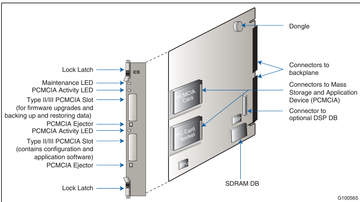
Figure 2 ICB card
