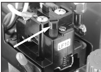
Figure 9. Pressure Regulator
