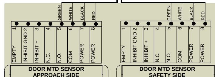
LO-LINX SUPERSCAN HARNESS p/n: 70.5071
