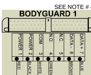
LO-LINX SUPERSCAN HARNESS p/n: 70.5071
