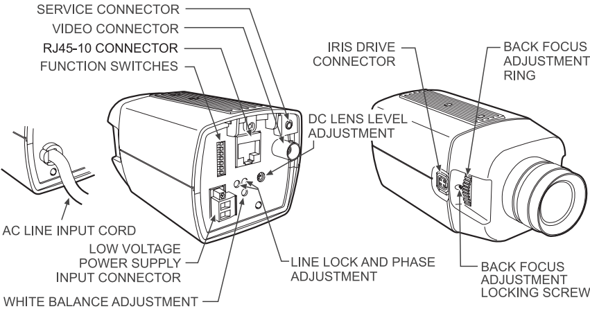
Figure 1. Camera Layout
