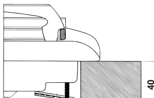
Clamp Position for H=40mm top
