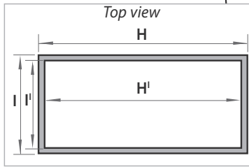
Product and cabinetry dimensions (mm)
