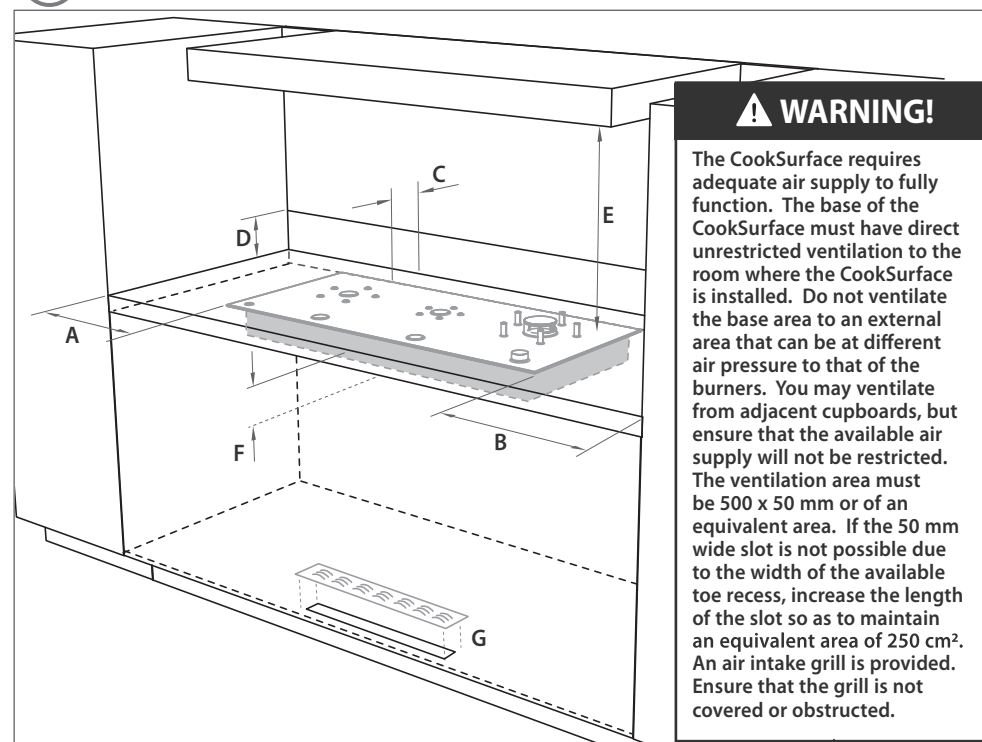
Clearances (mm)
