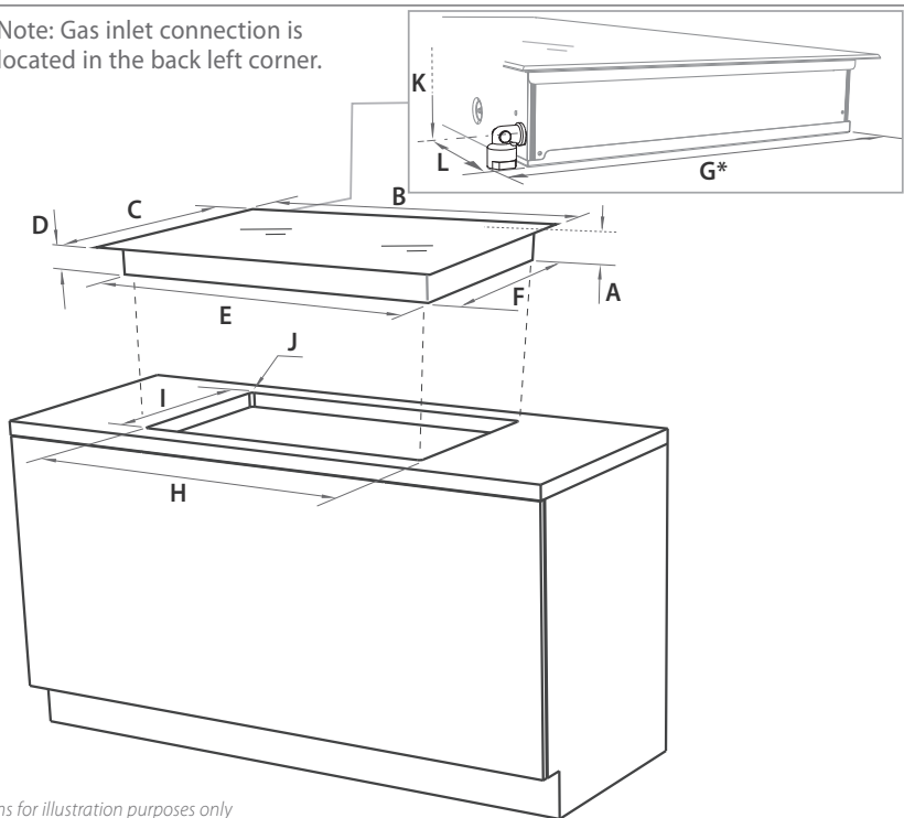
Product and cabinetry dimensions (mm)
