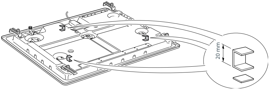
Fig. 3 Mounting the base clearance spacers
