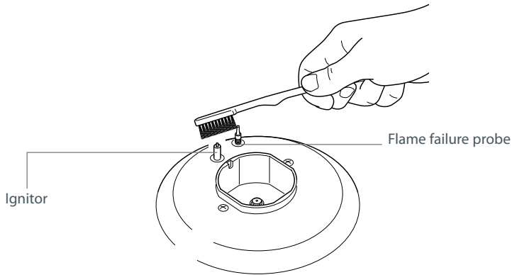
Fig.15 Cleaning the ignitor and probe
