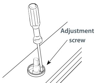
Fig. 9 Adjusting a burner's minimum gas rate setting
