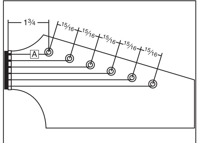
Figure 5. Peghole placement.
