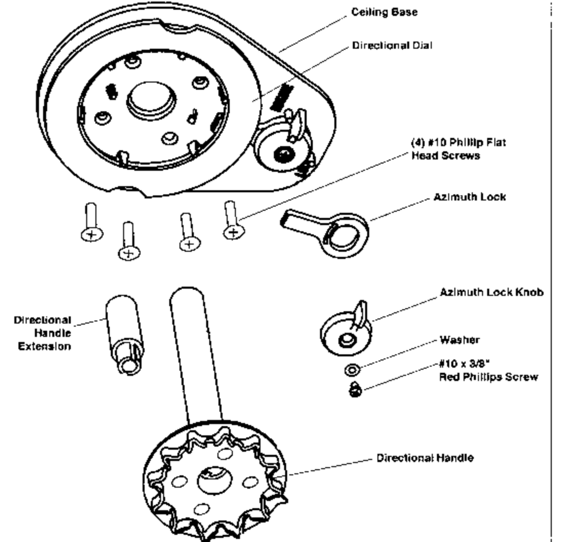
INTERIOR HARDWARE KIT RK-CEIL
