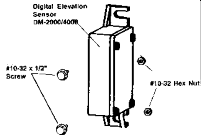
Sensor parts w/cable, installed at factory
