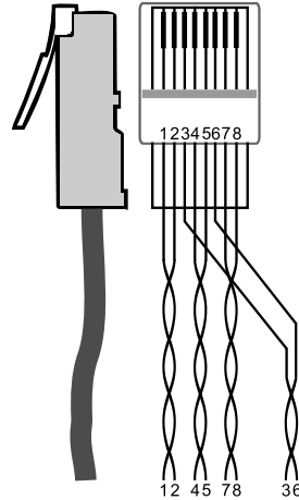
Figure 9: CAT 5 PINOUT
