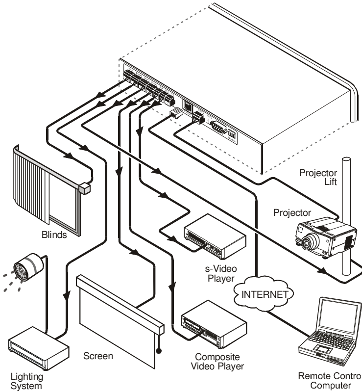
Figure 16: Example of a Typical Media/Room Controller Section Configuration
