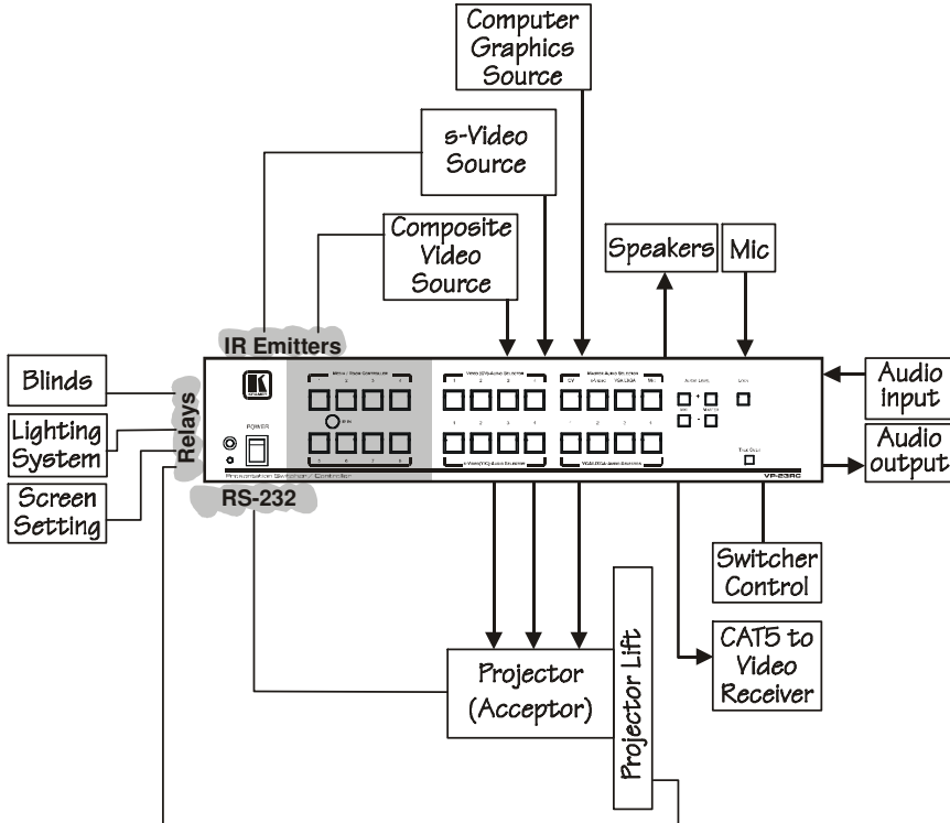
Figure 1: VP-23RC Configuration Example
