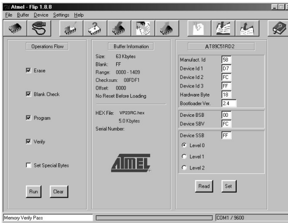
Figure 30: Atmel – Flip Window (Operation Completed)
