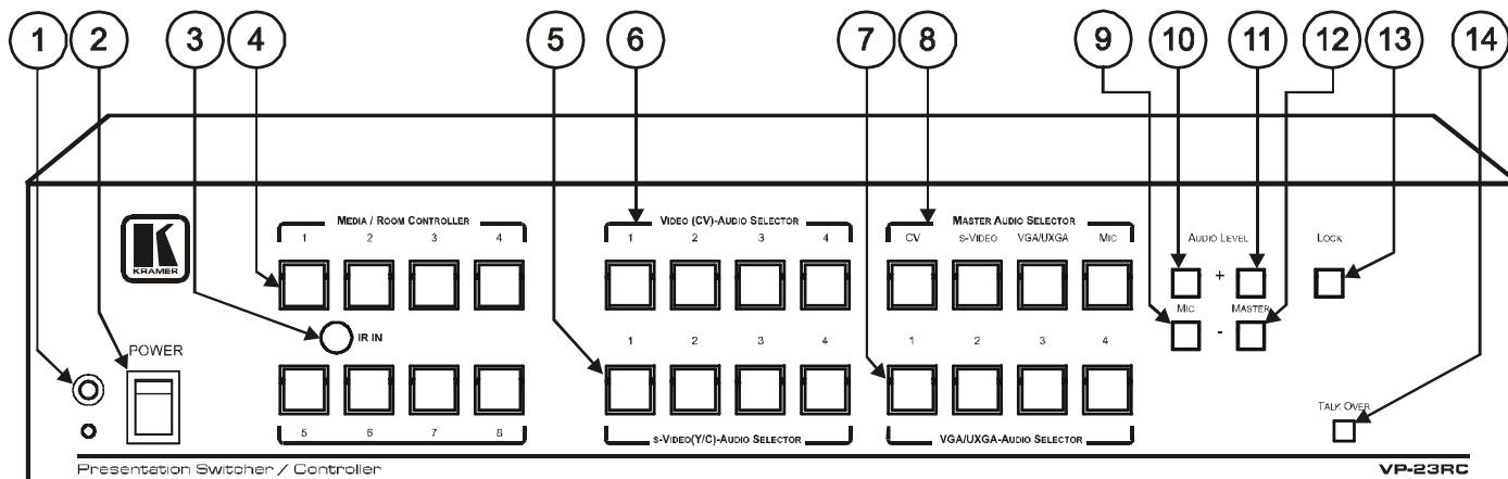
Figure 2: VP-23RC Presentation Switcher / Controller – Front View
