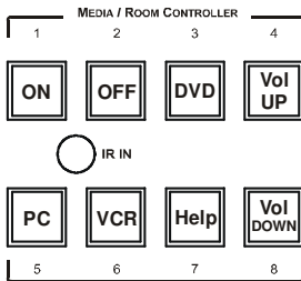
Figure 18: Labels Setup
