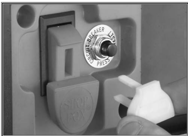
Figure 28. Remove the safety lockout key.
