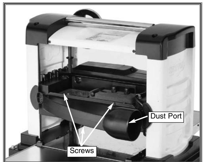
Figure 12. Dust port mounted to planer.
