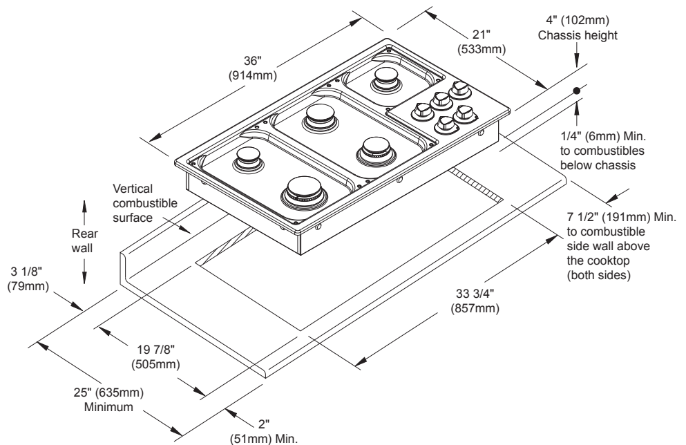
Cutout Dimensions for the PGM365-1
