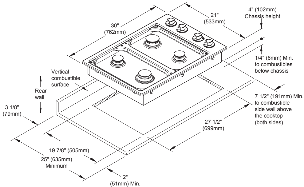
Cutout Dimensions for the PGM304-1
