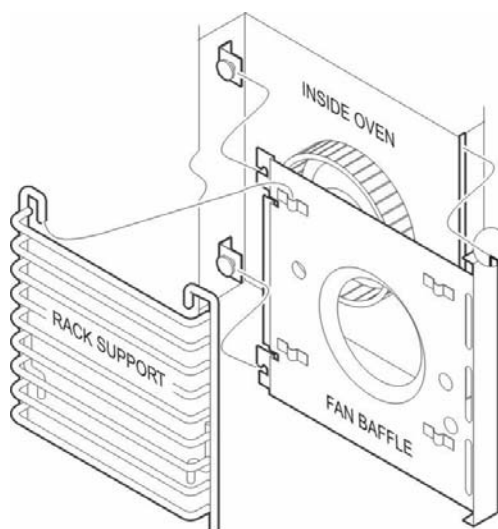
Fig. 7 Oven Rack Installation
