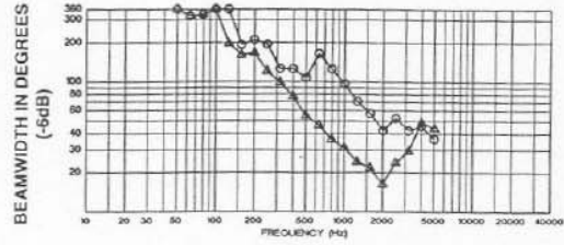
FIGURE 3 — TL15-2 One-Third-Octave Beamwidth vs Frequency (anechoic environment)
