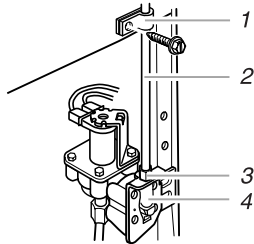
1. Tube Clamp 3. Compression Nut 2. Copper Tubing 4. Valve Inlet
