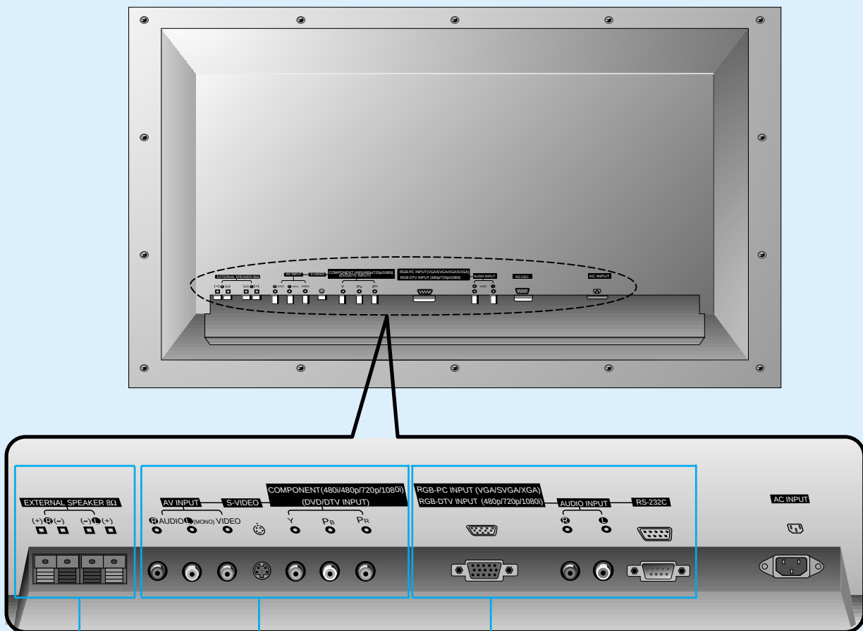
Back Panel
