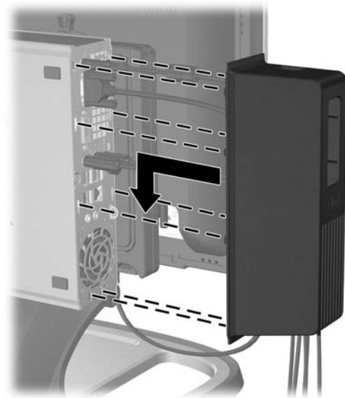
Figure 3-8 Installing the Port Cover
