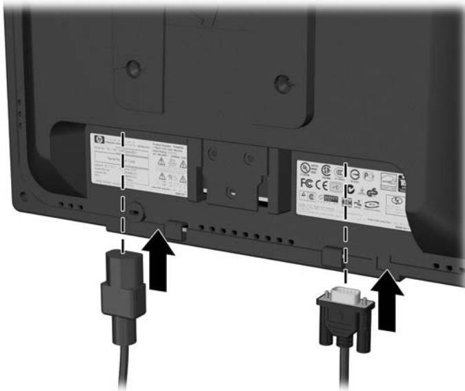
Figure 3-1 Connecting VGA and Power Cables to the Monitor
